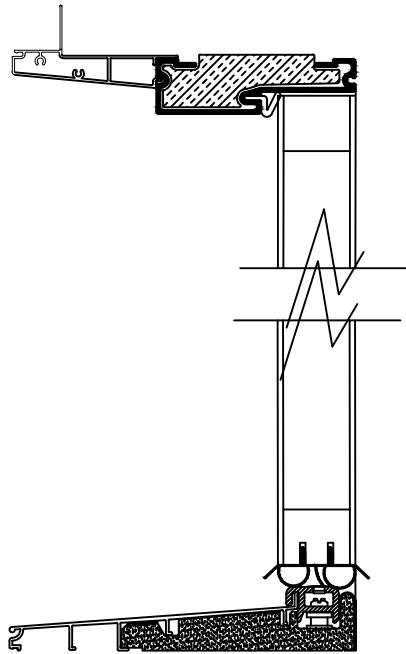
6 5/8" Fiberglass Frame Inswing Door
