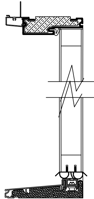
4 5/8" Fiberglass Frame Inswing Door
